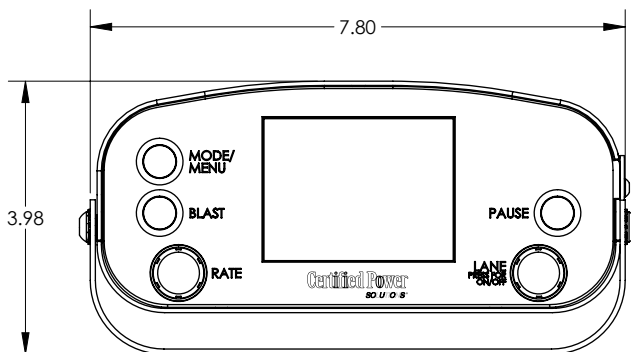
Mechanical layout
